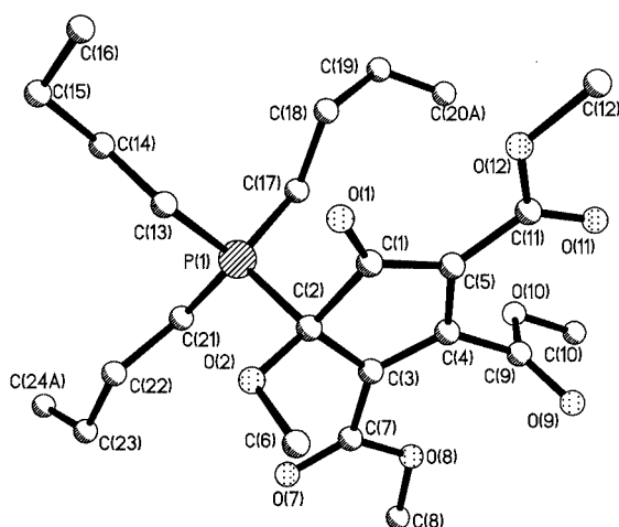
Figure 1. X-ray structure of the zwitterionic compound 2 showing crystallographic numbering scheme; selected bond lengths (Å) and angles ( ^\circ ): P(1)–C(2) 1.853(4), P(1)–C(21) 1.796(5), C(1)–C(2) 1.569(5), C(1)–O(1) 1.227(4), C(2)–C(3) 1.522(5), C(3)–C(4) 1.376(5), C(3)–C(7) 1.442(5), C(4)–C(5) 1.418(5), C(4)–C(9) 1.495(9), C(5)–C(1) 1.426(5), C(5)–C(11) 1.433(6), C(1)–C(2)–C(3) 103.0(3), C(2)–C(3)–C(4) 107.2(3), C(3)–C(4)–C(5) 114.0(3), C(4)–C(5)–C(1) 107.9(3), C(5)–C(1)–C(2) 107.0(3).
